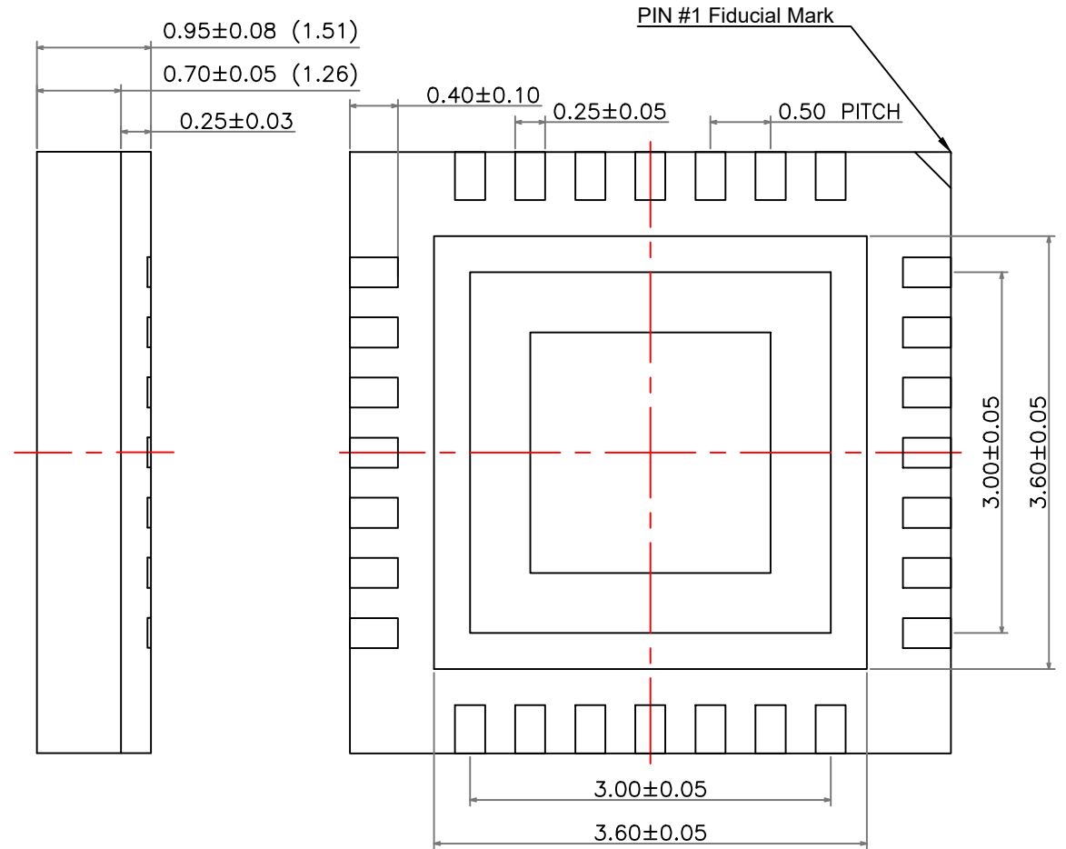
SIDE VIEW
